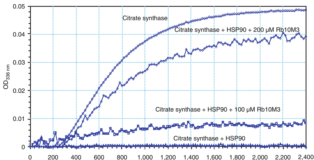
Fig. 24.5 Dose-dependent inhibition by Rb10M3 of HSP90 chaperone function using a citrate synthase aggregation assay. Rb10M3 is a derivative of Rb10 with dA (A2dA) to increase stability. Citrate synthase (0.115 \mu M),
